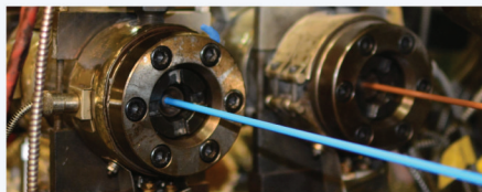
Extruder in production
