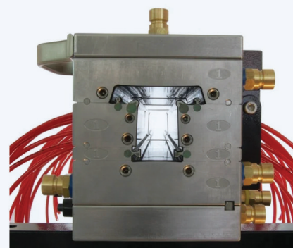
Tooling-Mold/Dies for making profiles
